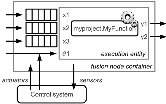
Fig. 3. Implementation details - Fusion node implementation.
