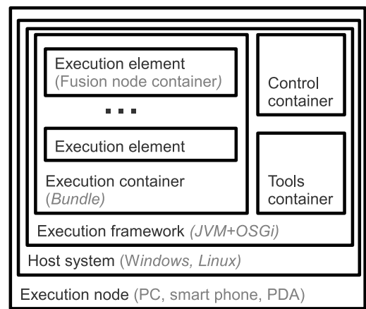
Fig. 2. Implementation details - Runtime frameworks hierarchy.
