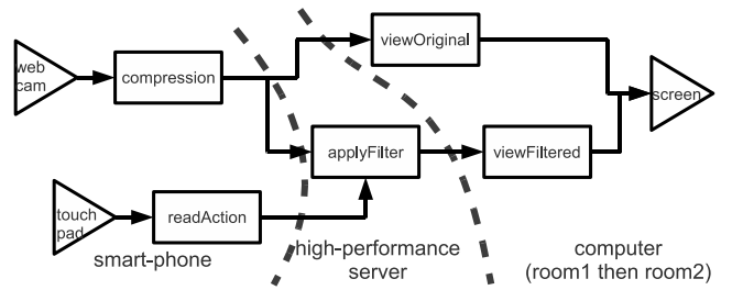
Fig. 5. Passer-by example of reconfiguration - process view.
